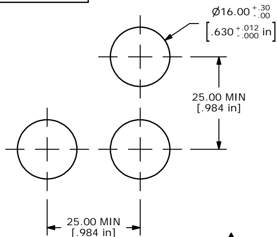
PANEL MOUNTING
