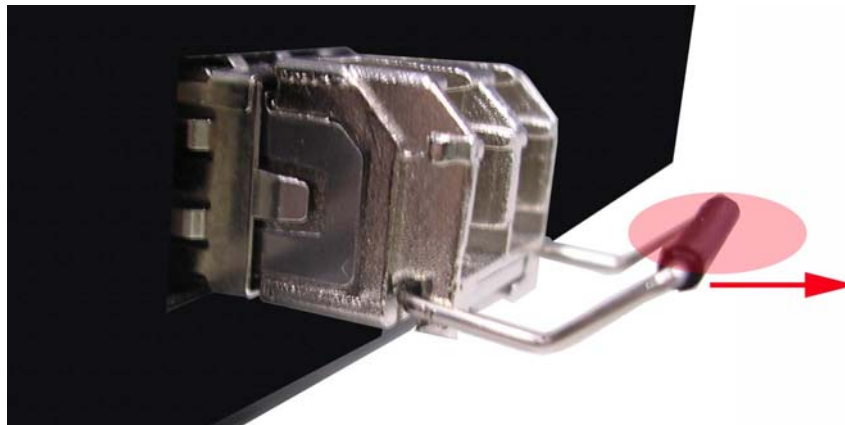
Figure 2.12: Pull out from the transceiver
