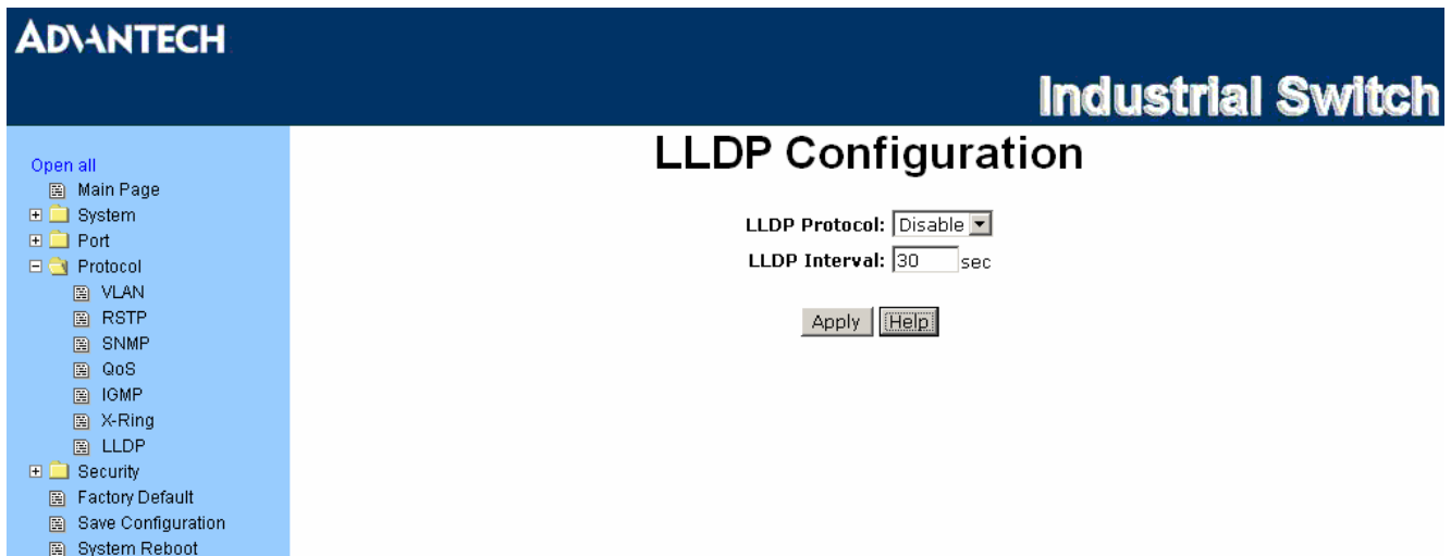
Figure 3.58: LLDP Configuration interface
