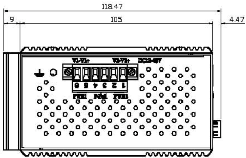
Figure 2.4: Top View of EKI-2748CI
