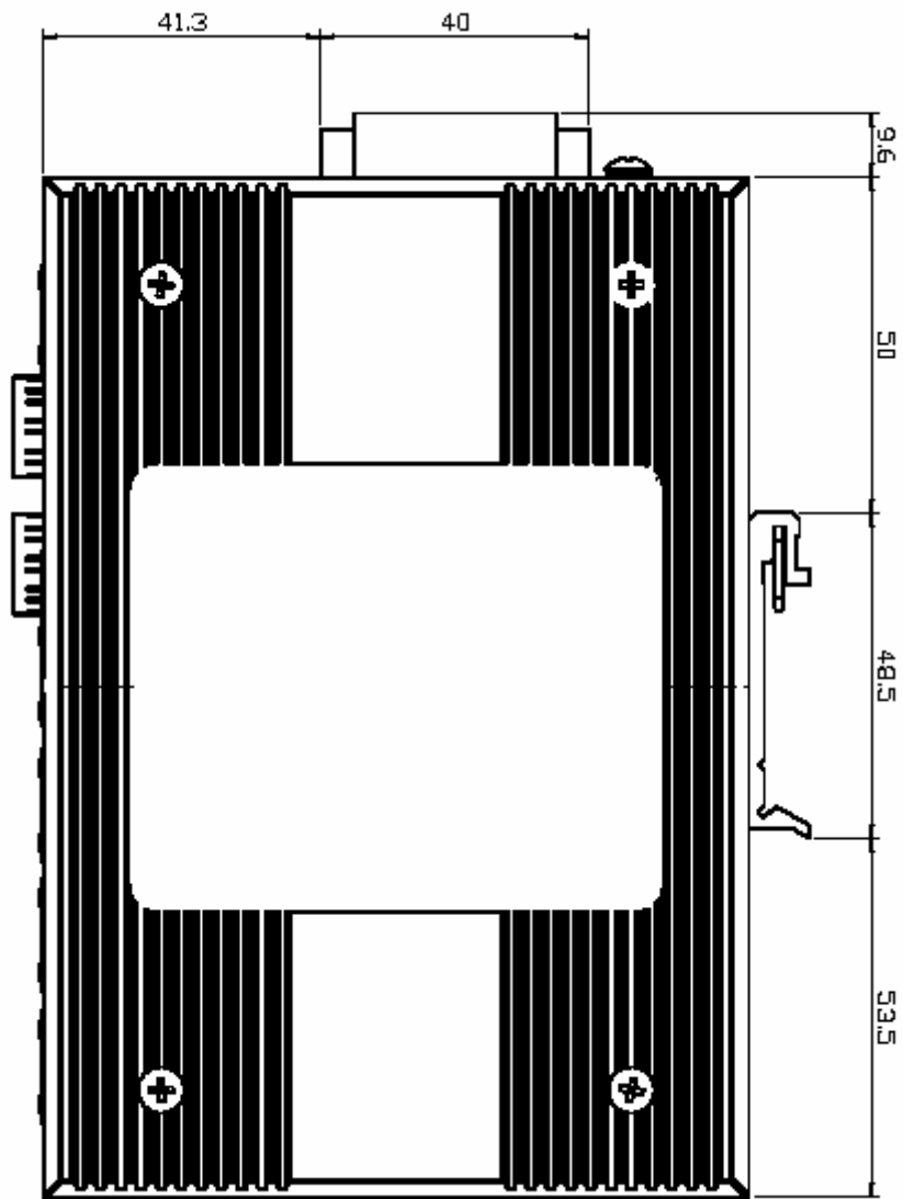
Figure 2.2: Side View of EKI-2748CI
