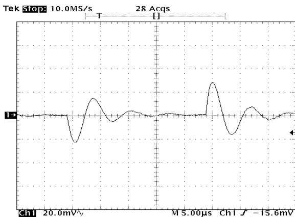
FIGURE 24. LINE TRANSIENT RESPONSE, 0.001µF LOAD CAPACITANCE
