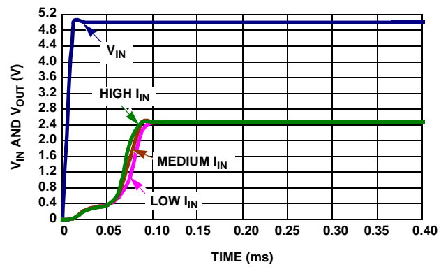
FIGURE 25. TURN-ON TIME
