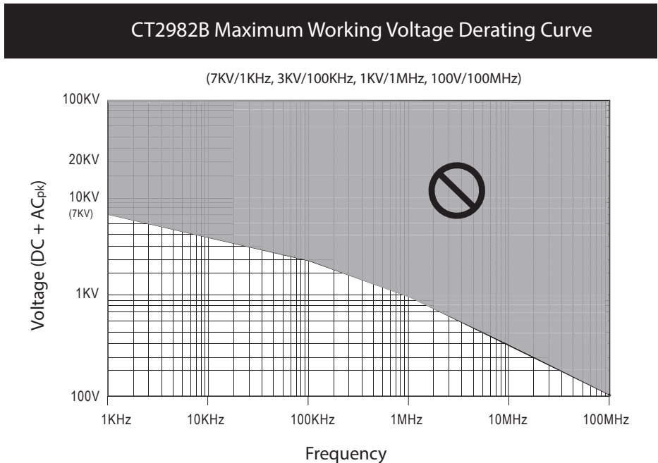
Figure 4: Voltage Derating Curve
