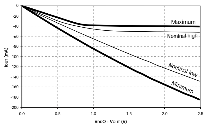
Figure 8: Normal Drive Pull-Up Characteristics
