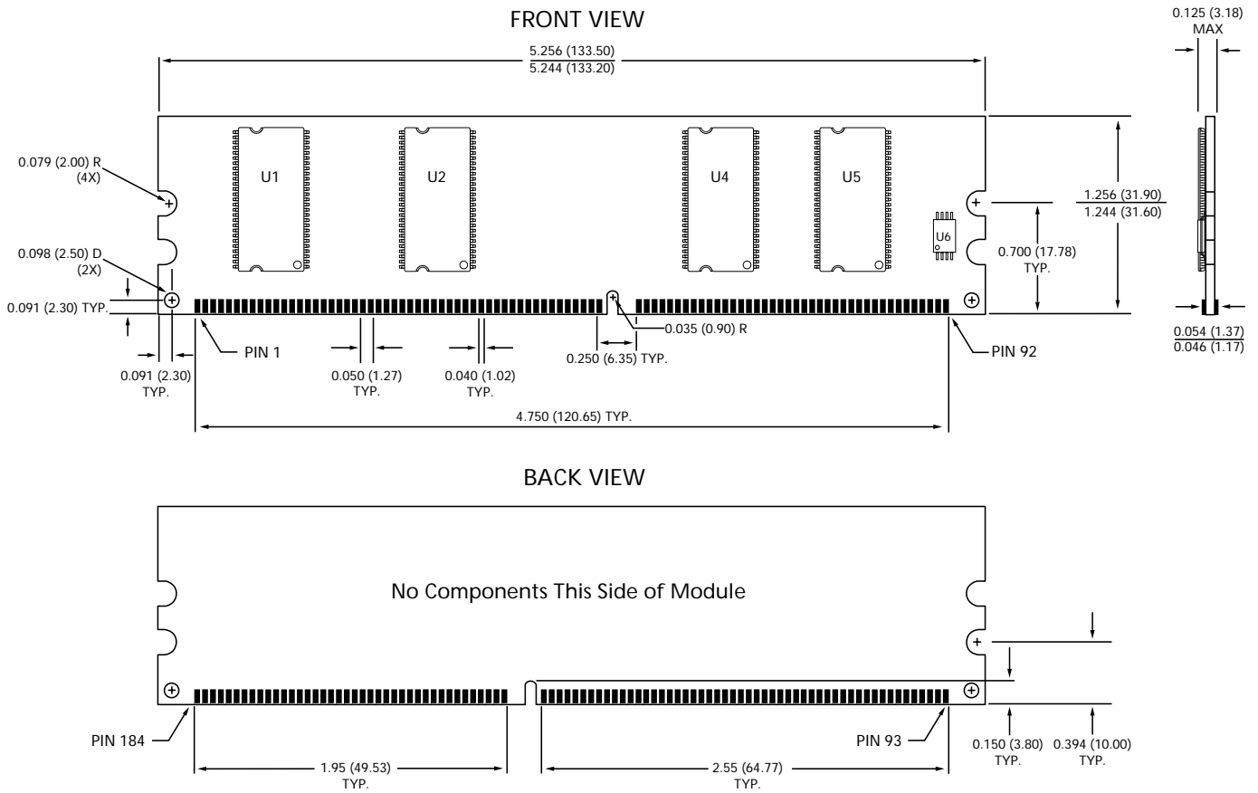
Figure 16: 184-Pin DIMM Dimensions
