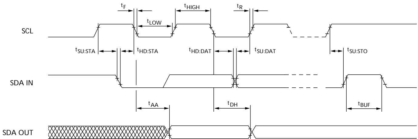
Figure 15: SPD EEPROM Timing Diagram
