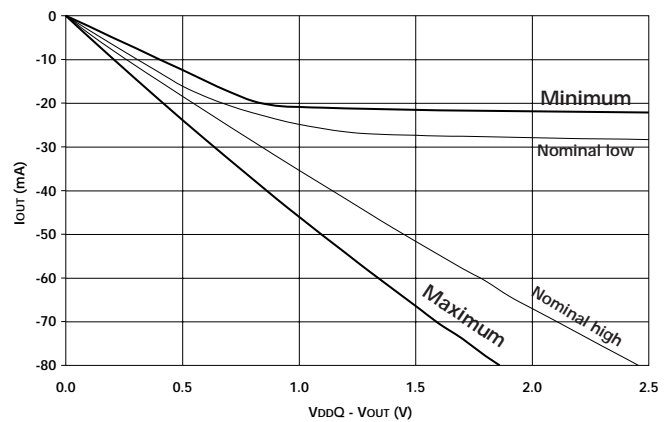
Figure 10: Reduced Drive Pull-Up Characteristics
