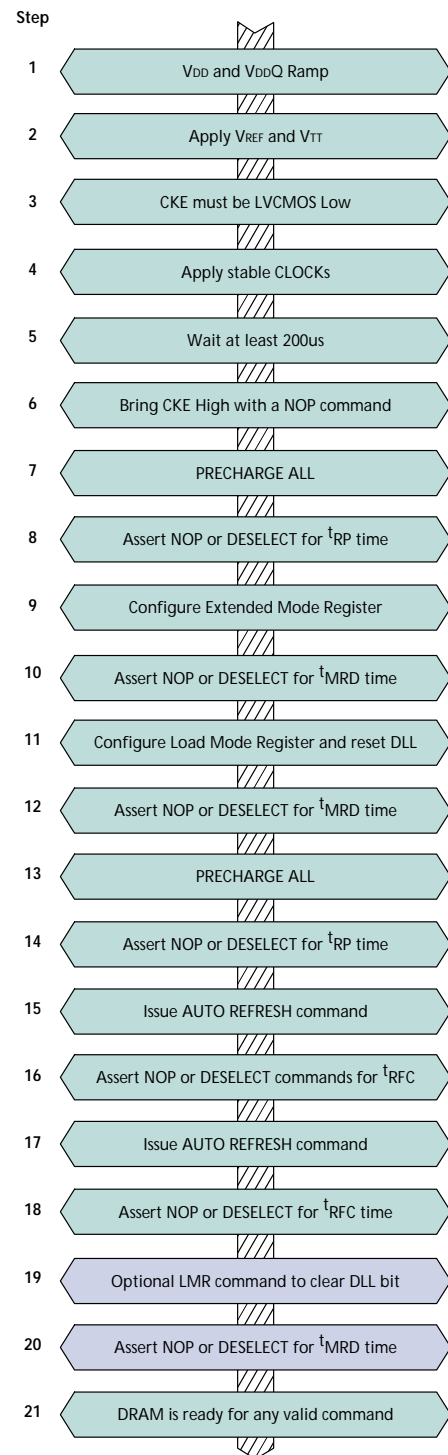
Figure 11: Initialization Flow Diagram
