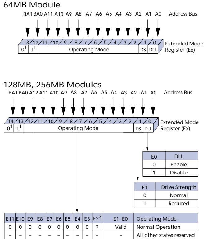
Figure 5: Extended Mode Register Definition Diagram
