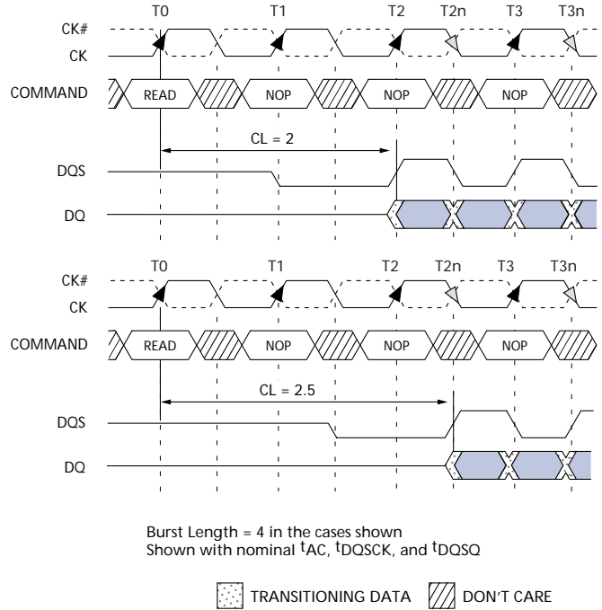
Figure 4: CAS Latency Diagram
