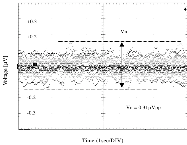
0.1Hz to 10Hz Noise
