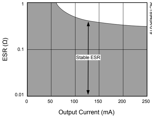
Region of Stable C OUT ESR vs. Output Current
