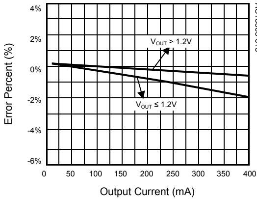
REG4, 5, 6, 7 Output Voltage vs. Output Current
