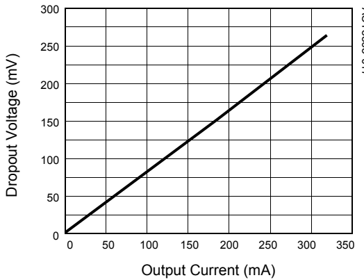
REG5, 7 Dropout Voltage vs. Output Current
