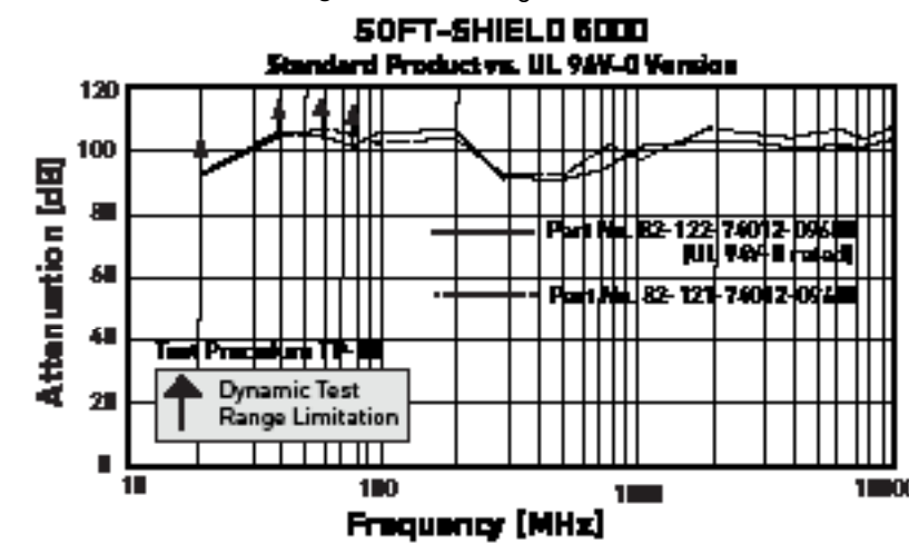
Figure 1 Shielding Effectiveness
