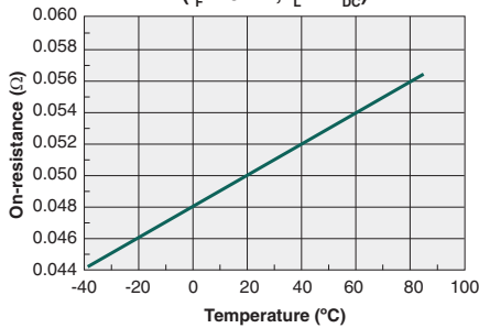
Typical On-Resistance vs. Temperature ( I_F=10\text{mA} , I_L=1A_{DC} )
