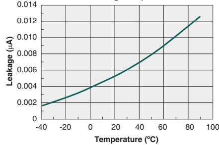
Typical Leakage vs. Temperature Measured Across Pins 1&2 ( V_L=60V_p )
