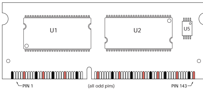
Figure 2: 144-Pin SODIMM Pin Locations
