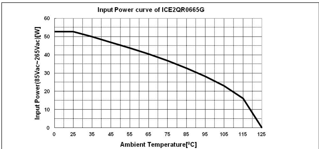
Figure 13 Input Power curve V_{in}=85\sim 265\text{Vac} ; P_{in}=f(T_a)
