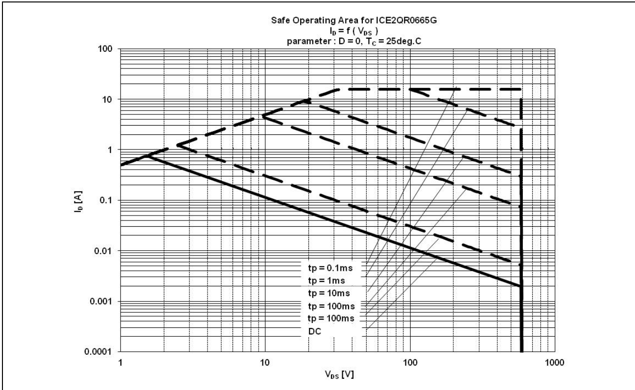
Figure 10 Safe Operating Area (SOA) curve for ICE2QR0665G
