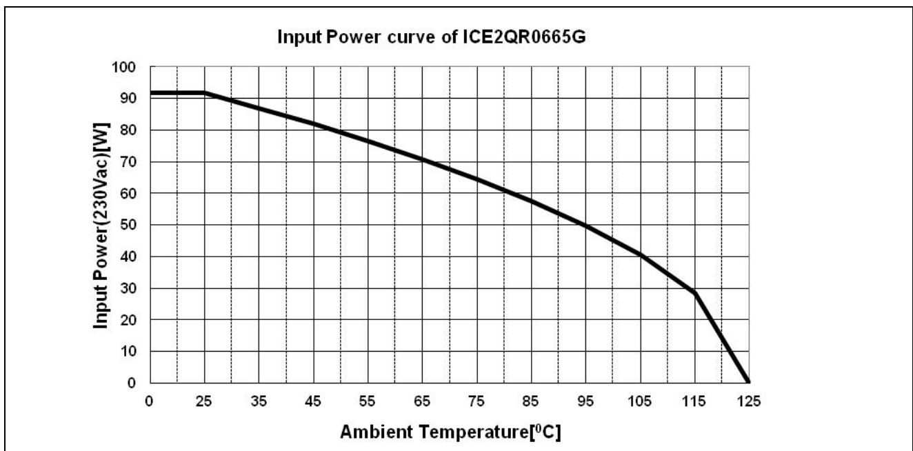
Figure 14 Input Power curve V_{in}=230\text{Vac} ; P_{in}=f(T_a)
