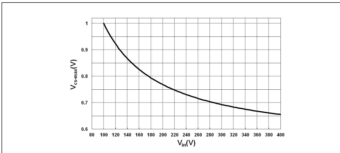
Figure 7 Variation of the V_{CS} limit voltage according to the I_{ZC} current
