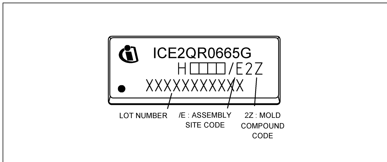
Figure 16 Marking for ICE2QR0665G
