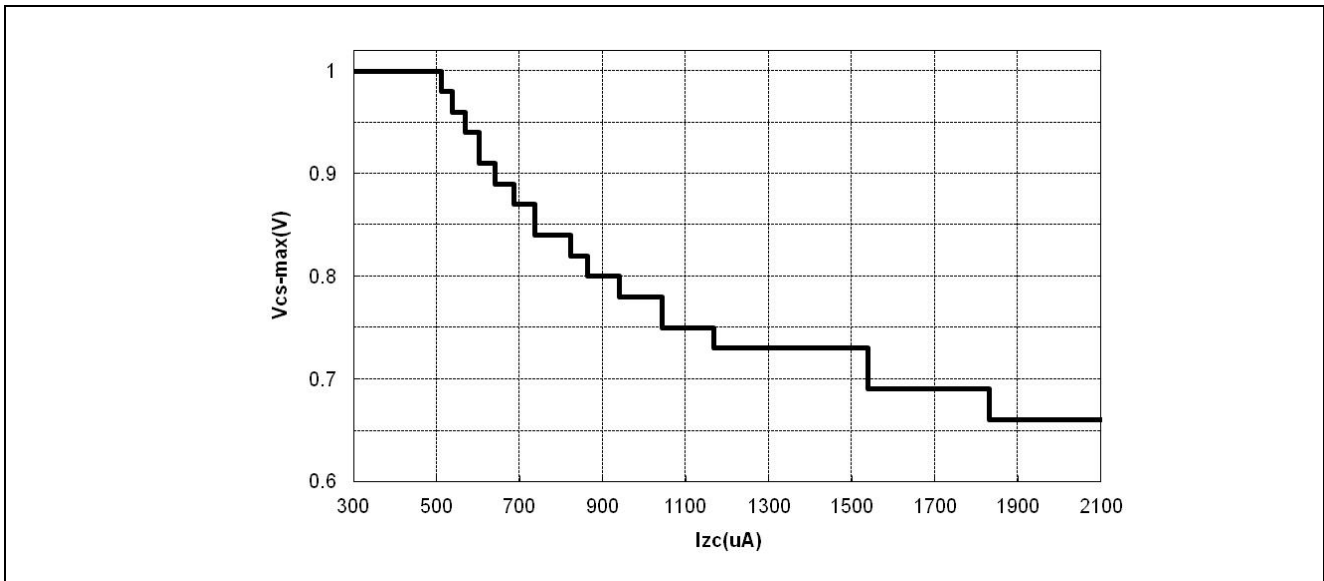
Figure 8 V CS-max versus I ZC
