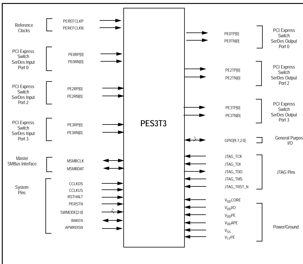
Figure 1.2 PES3T3 Logic Diagram
