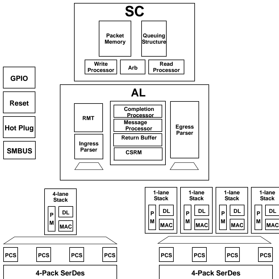
Figure 1.1 PES3T3 Architectural Block Diagram
