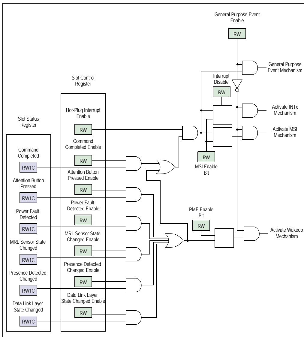
Figure 8.4 PES3T3 Hot-Plug Event Signalling
