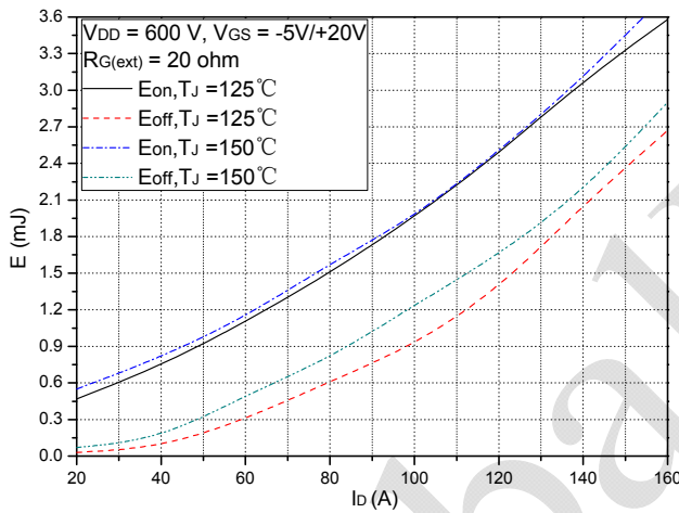
Fig.3 Typical Switching Loss vs. Collector Current
