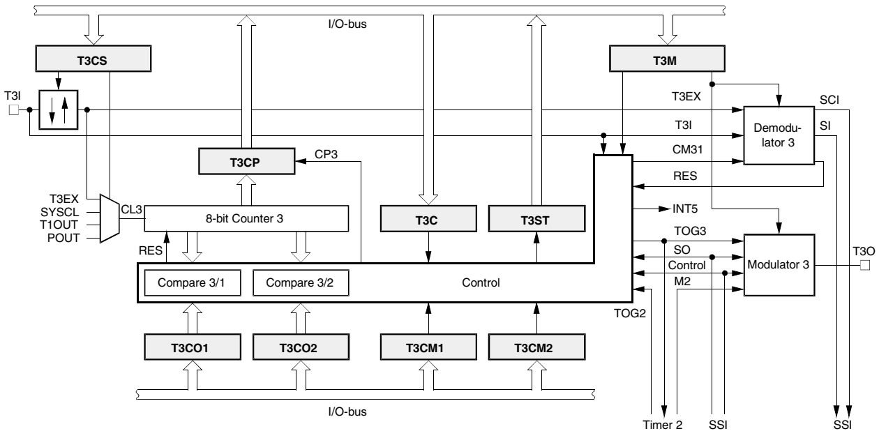
Figure 5-24. Timer 3
