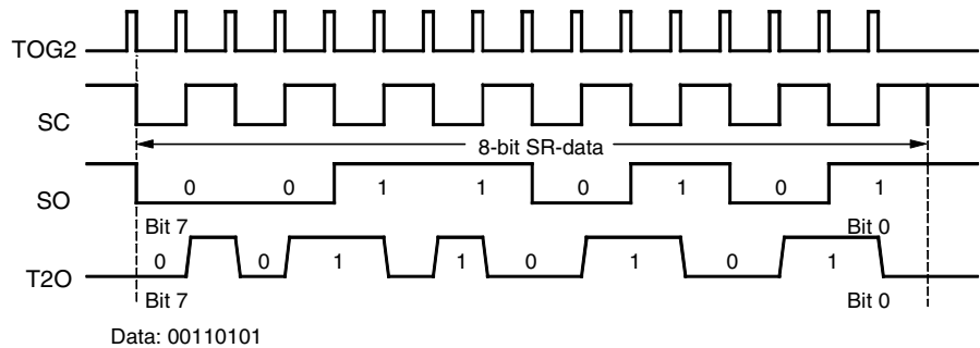
Figure 5-51. Manchester Modulation 1
