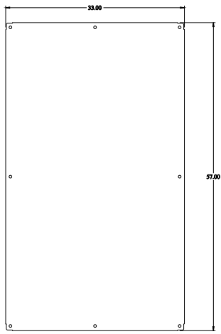
INNER PANEL
